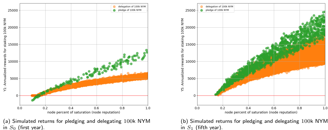
Fig. 16: Simulated annual rewards when pledging and delegating 100k NYM in the considered scenario.
