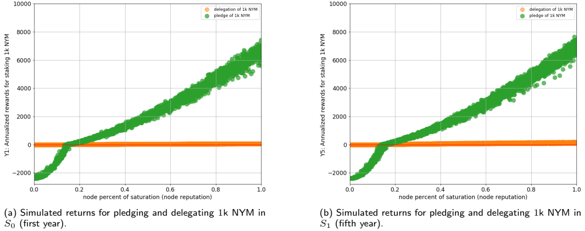
Fig. 14: Simulated annual rewards when pledging and delegating 1k NYM in the considered scenario.
