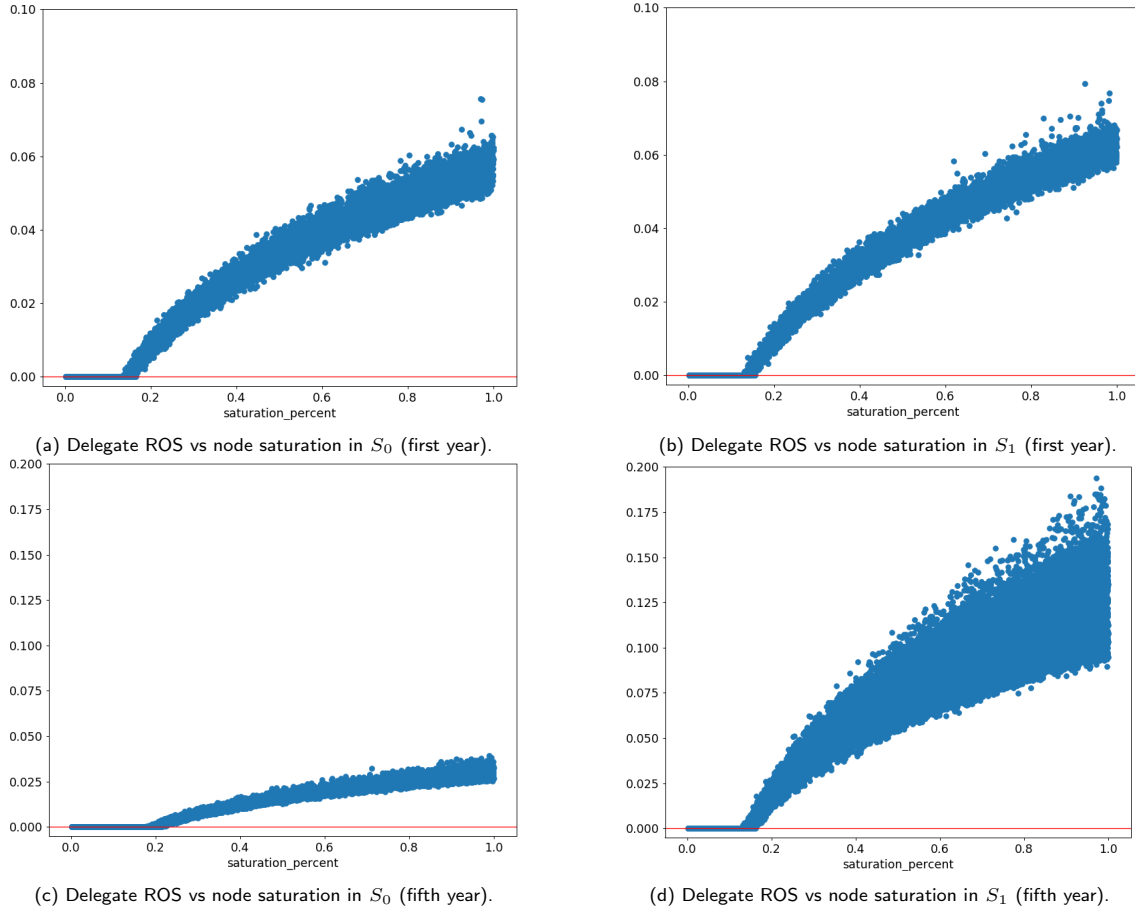
Fig. 13: Scatterplot of ROS (Return On Stake) vs node saturation, in S_0 and S_1 in the first and fifth years of operation.
