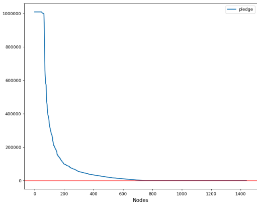
(a) Distribution of node pledges in a network with K = 720 , N = 1440 , and 15% of available token supply dedicated to pledging. Ordered by pledge.
